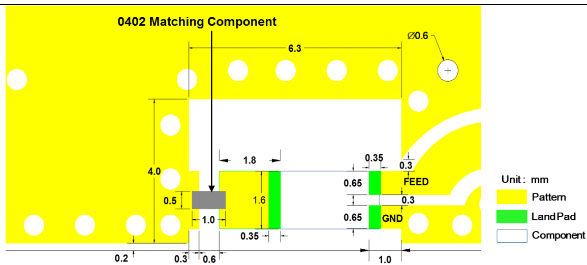
Land Pattern
