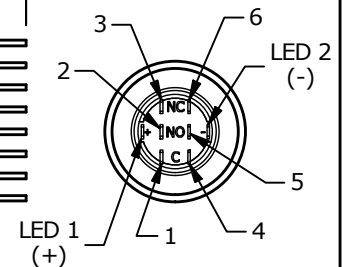
BOTTOM VIEW SHOWN WITHOUT WIRING AND DETACHABLE SOCKET
