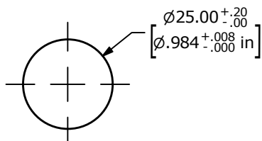
RECOMMENDED PANEL CUTOUT MAX. PANEL THICKNESS 10.0 [.39 in]
