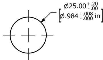
RECOMMENDED PANEL CUTOUT MAX. PANEL THICKNESS 10.0 [.39 in]
