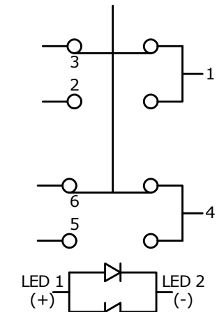
SCHEMATIC ▲ ON - (ON) DPDT Illuminated ( ) DENOTES MOMENTARY FUNCTION
