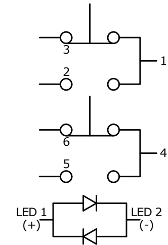
SCHEMATIC ▲ ON - (ON) DPDT Illuminated ( ) DENOTES MOMENTARY FUNCTION
