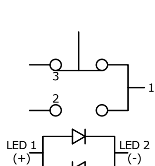
SCHEMATIC ▲ ON - ON SPDT Illuminated
