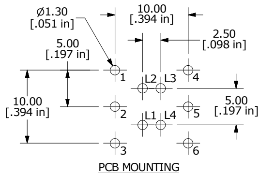
PCB MOUNTING
