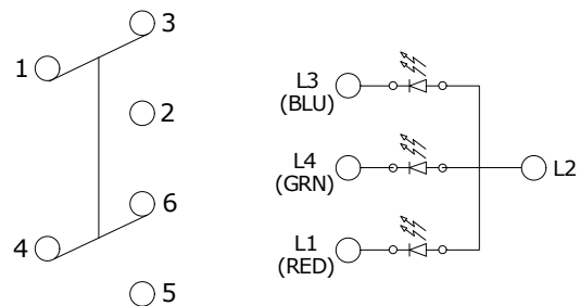
SWITCH SCHEMATIC LATCHING
