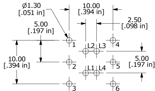
PCB MOUNTING
