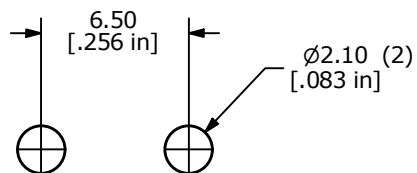
PANEL MOUNTING
