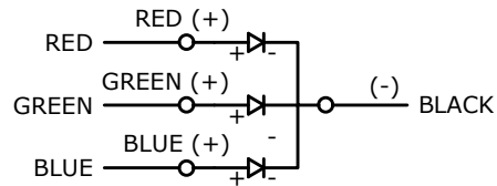
SCHEMATIC ON - ON - DPDT ILLUMINATED
