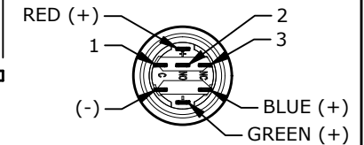
BOTTOM VIEW SHOWN WITHOUT WIRING
