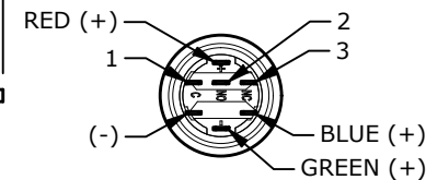
BOTTOM VIEW SHOWN WITHOUT WIRING
