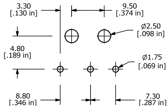
P.C. MOUNTING
