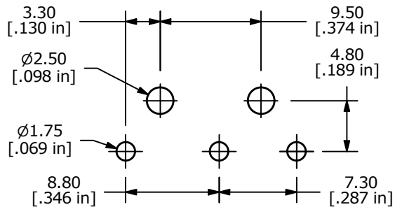
P.C. MOUNTING
