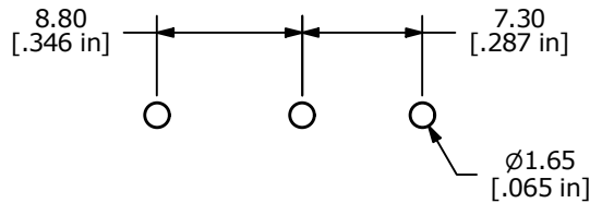
P.C. MOUNTING
