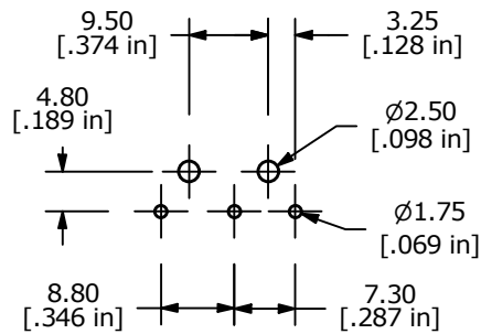
P.C. MOUNTING
