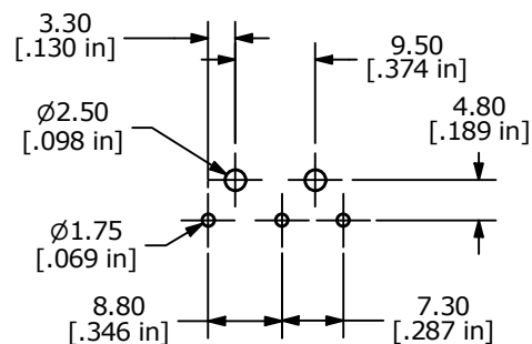
P.C. MOUNTING
