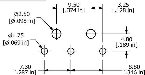
P.C. MOUNTING
