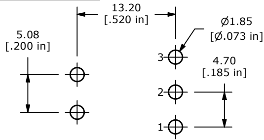
P.C. MOUNTING
