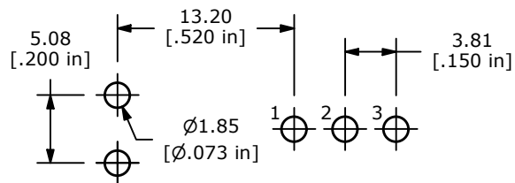
P.C. MOUNTING
