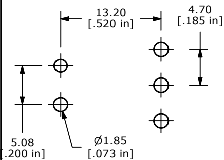
P.C. MOUNTING
