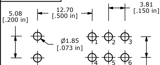
P.C. MOUNTING
