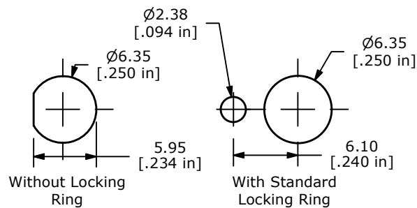
P.C. MOUNTING
