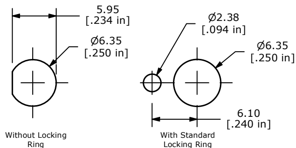
PANEL MOUNTING
