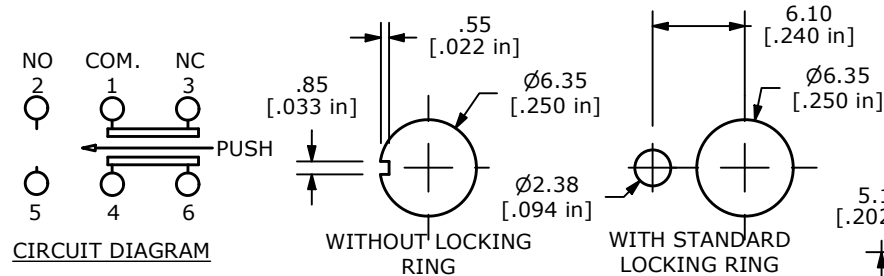
PANEL MOUNTING
