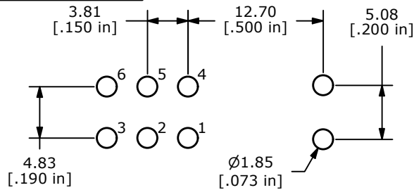
P.C. MOUNTING
