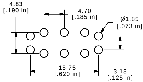
P.C. MOUNTING
