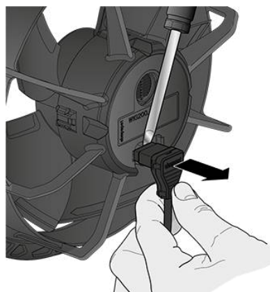
Fig. 3: Use a screwdriver to loosen the plug connection. With this, the plug can be levered out straight. Caution! The connections on the fan may be damaged if pulled out at an angle!
