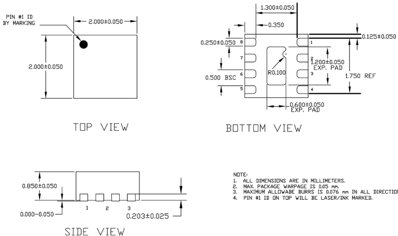
8-Pin Ultra-Small EPAD DFN
