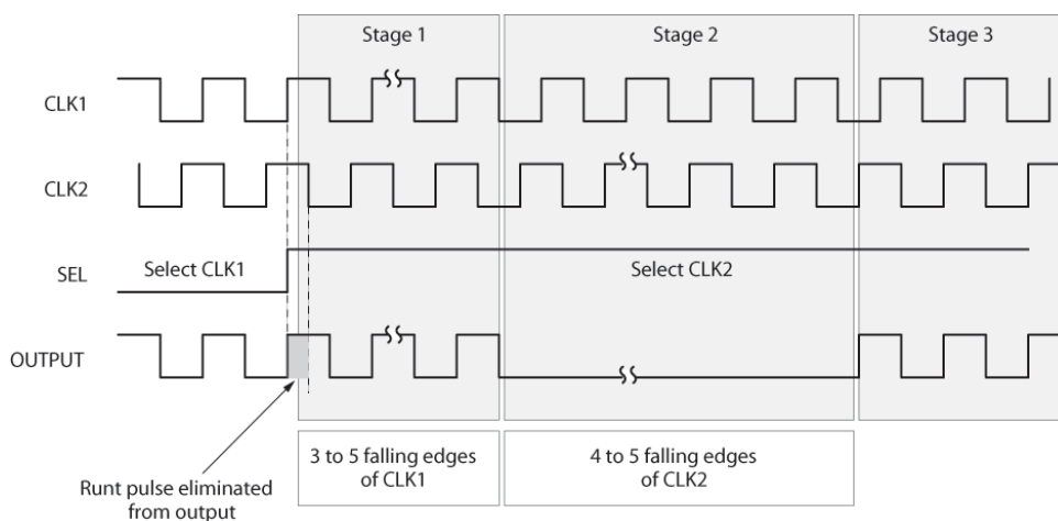
Figure 2. Timing Diagram 1
