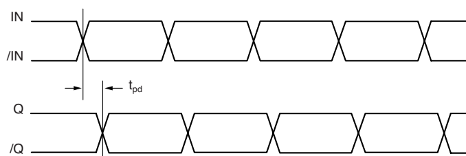
Figure 2. Timing Diagram
