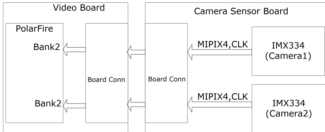
Figure 7 • MIPI-RX Connection
