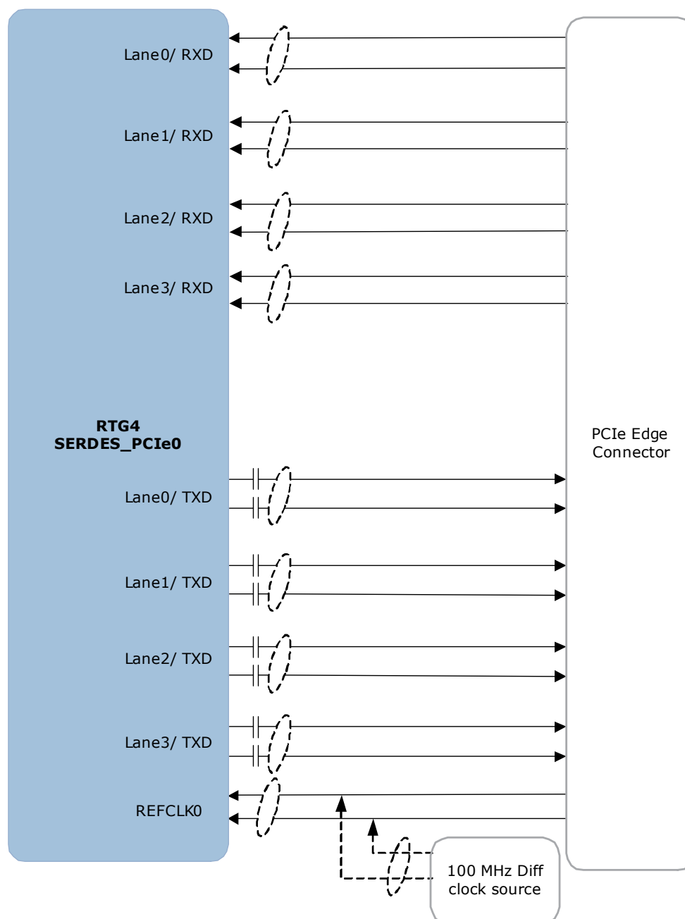
Figure 7 • SERDES_PClE0 Interface
