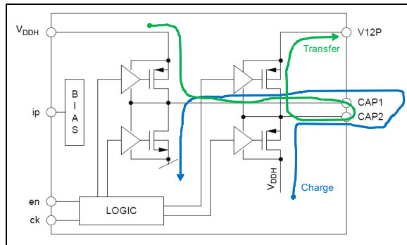
FIGURE 14-7: CHARGE PUMP
