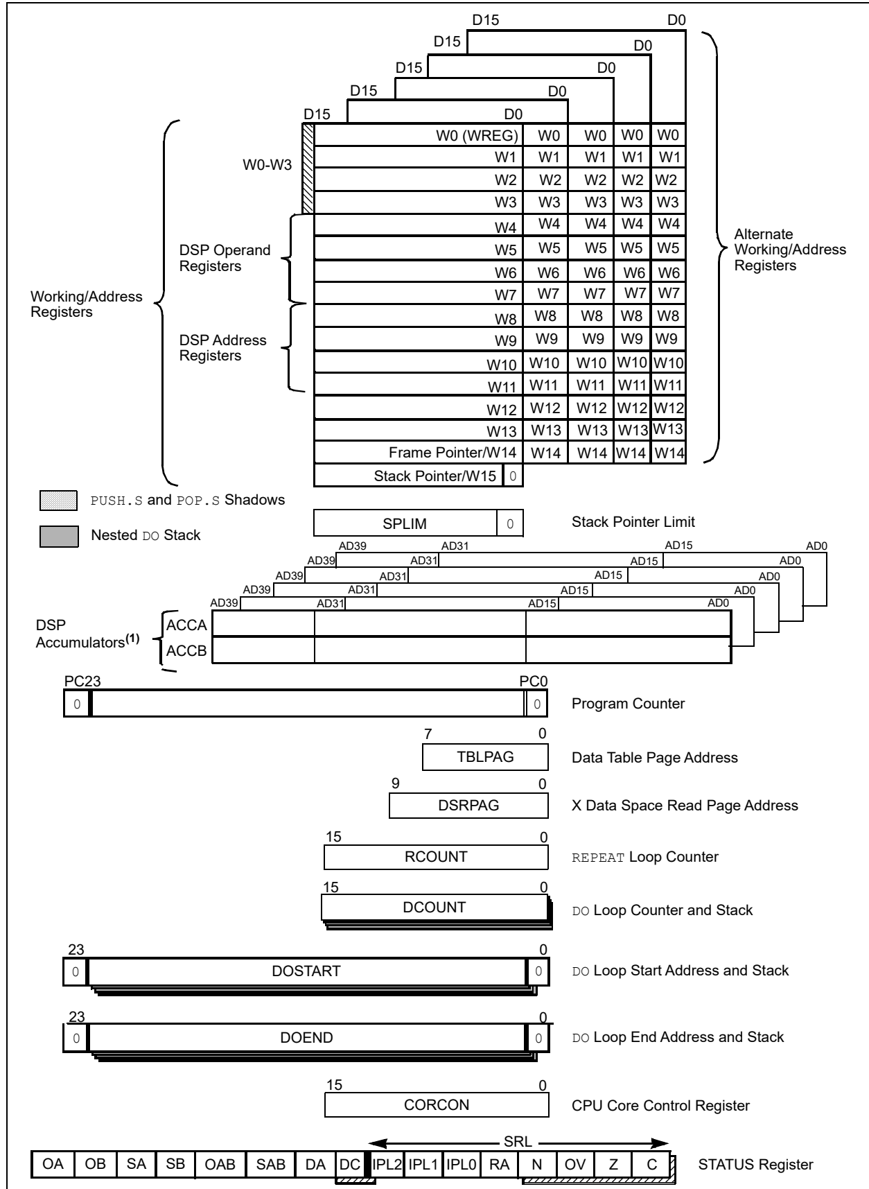
FIGURE 3-2: PROGRAMMER'S MODEL
