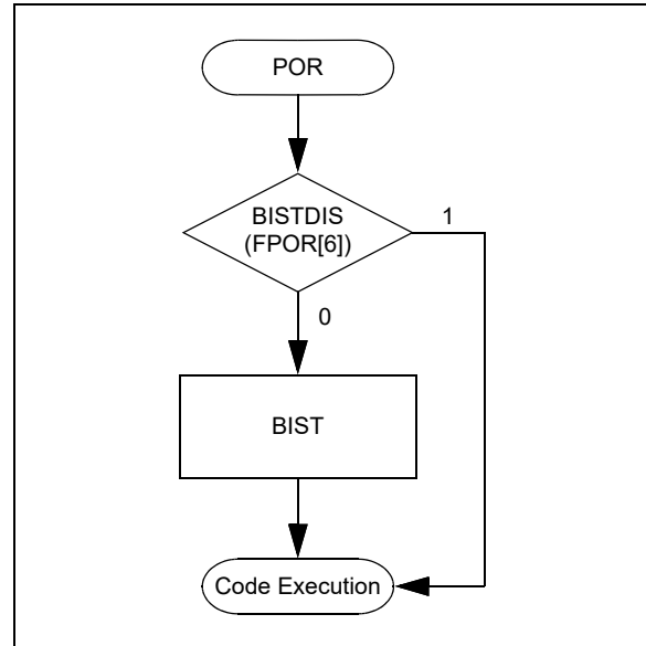
FIGURE 4-7: BIST FLOWCHART
