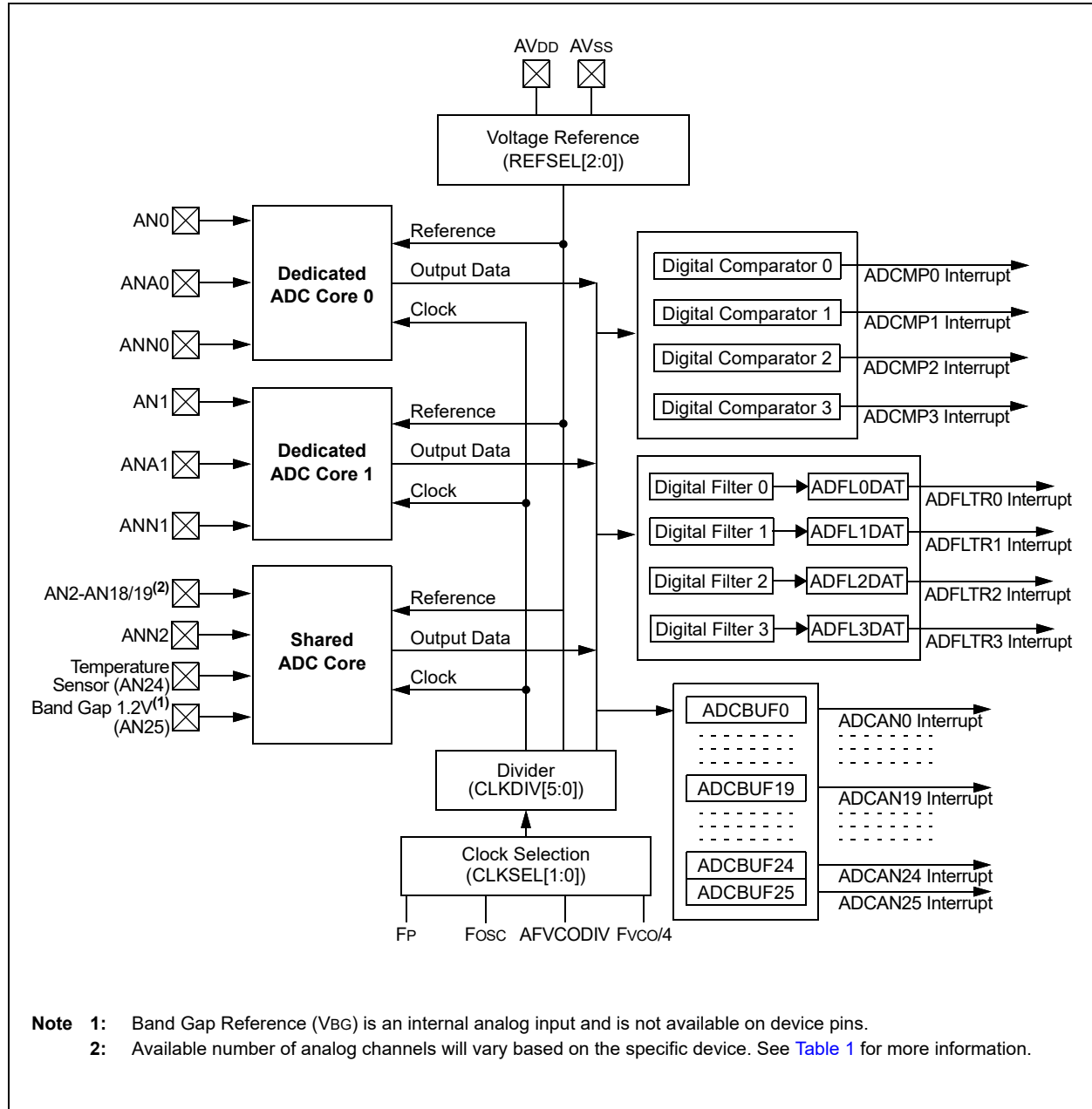
FIGURE 15-1: ADC MODULE BLOCK DIAGRAM
