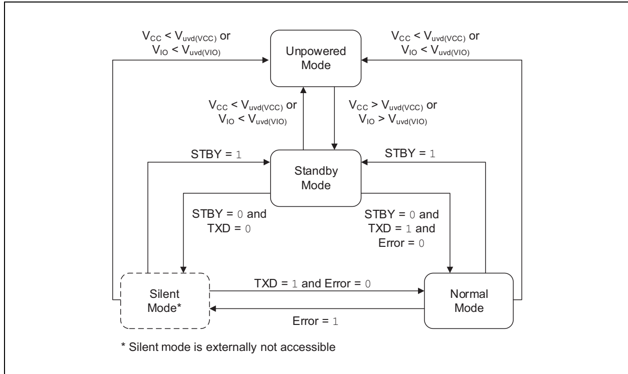
FIGURE 12-2: OPERATING MODES
