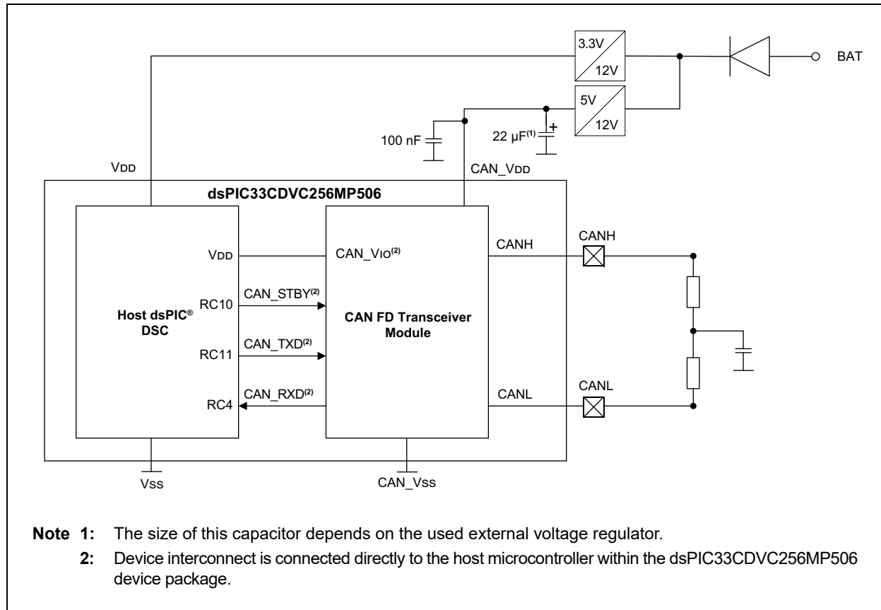
FIGURE 12-7: TYPICAL APPLICATION
