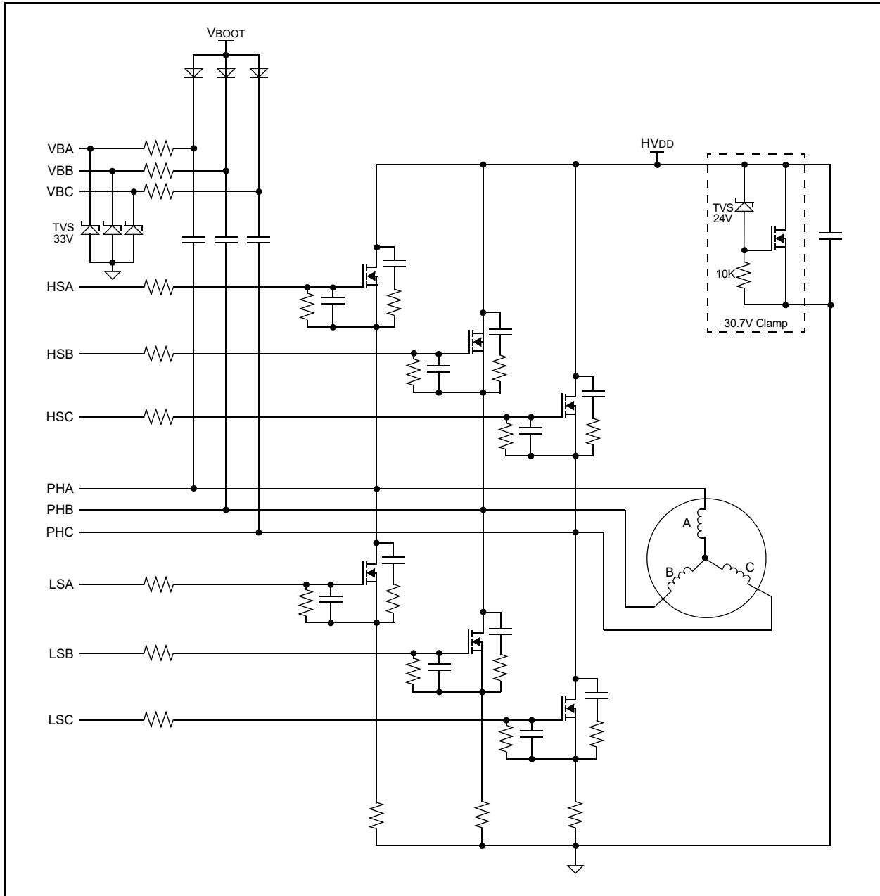
FIGURE 14-9: OVERVOLTAGE PROTECTION
