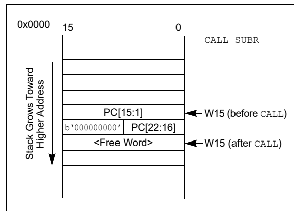
FIGURE 4-10: CALL STACK FRAME
