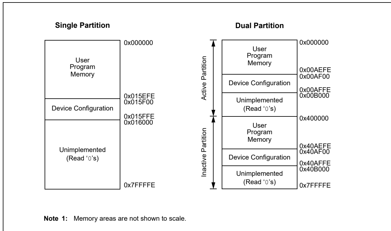
FIGURE 4-3: PROGRAM MEMORY MAP FOR dsPIC33CDVC128MP506 AND dsPIC33CDV128MP506/206 DEVICES (1)
