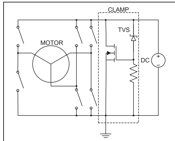
FIGURE 14-8: TRANSIENT VOLTAGE CLAMP
