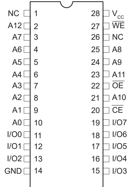
28-Lead SOIC
