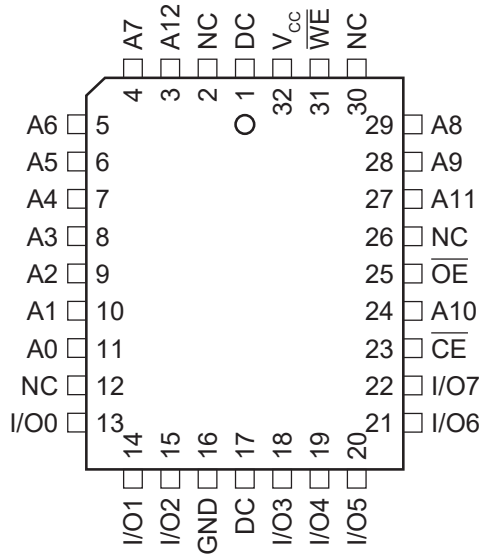
32-Lead PLCC
