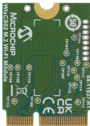
Figure 2-2. WlxC502 M.2 Wi-Fi® Module Card (EV59Y78A) – Bottom View
