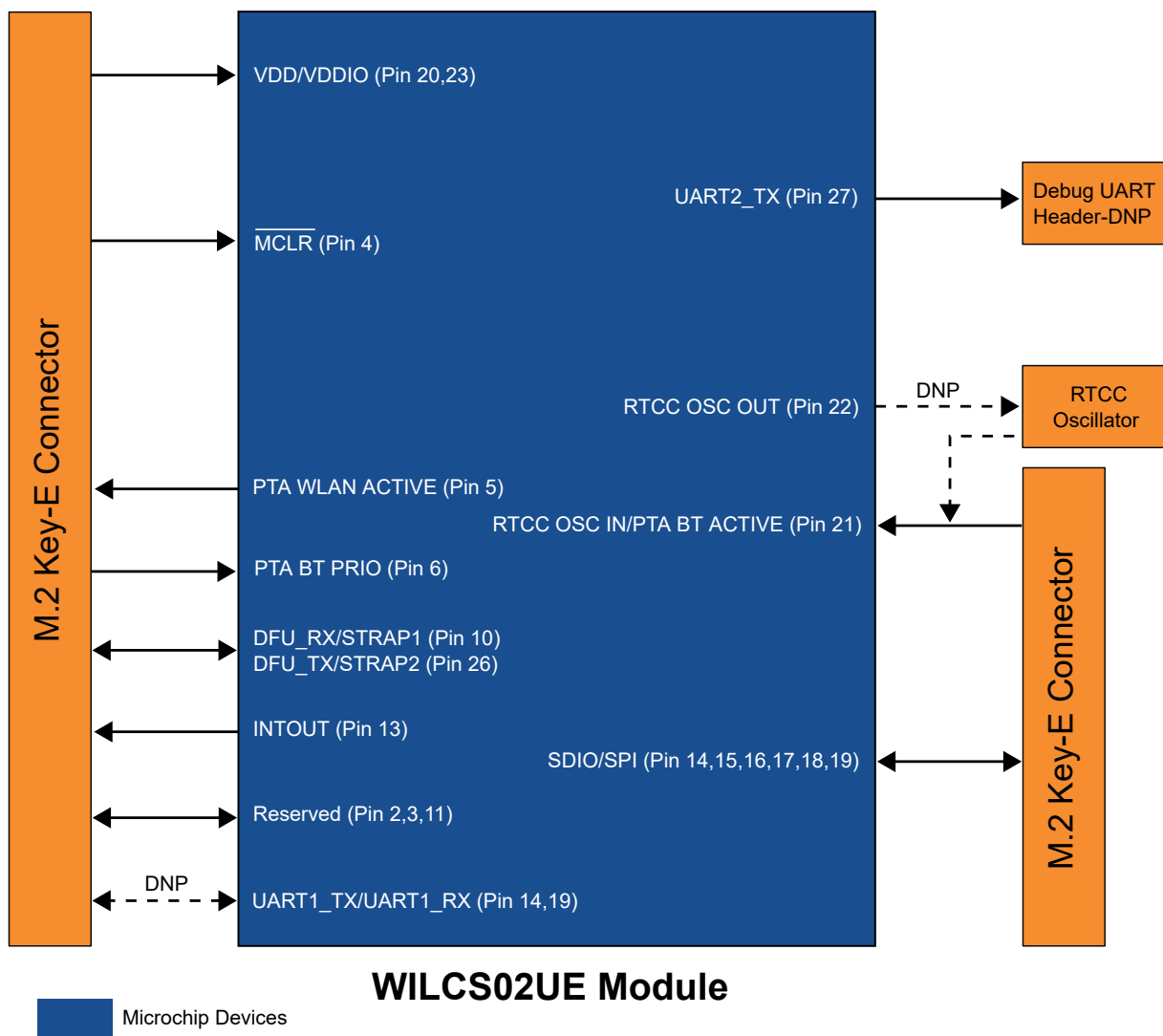
Figure 3-1. WlxC02 M.2 Wi-Fi® Module Card Block Diagram
