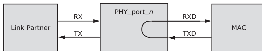
FIGURE 3-12: NEAR-END LOOPBACK DIAGRAM
