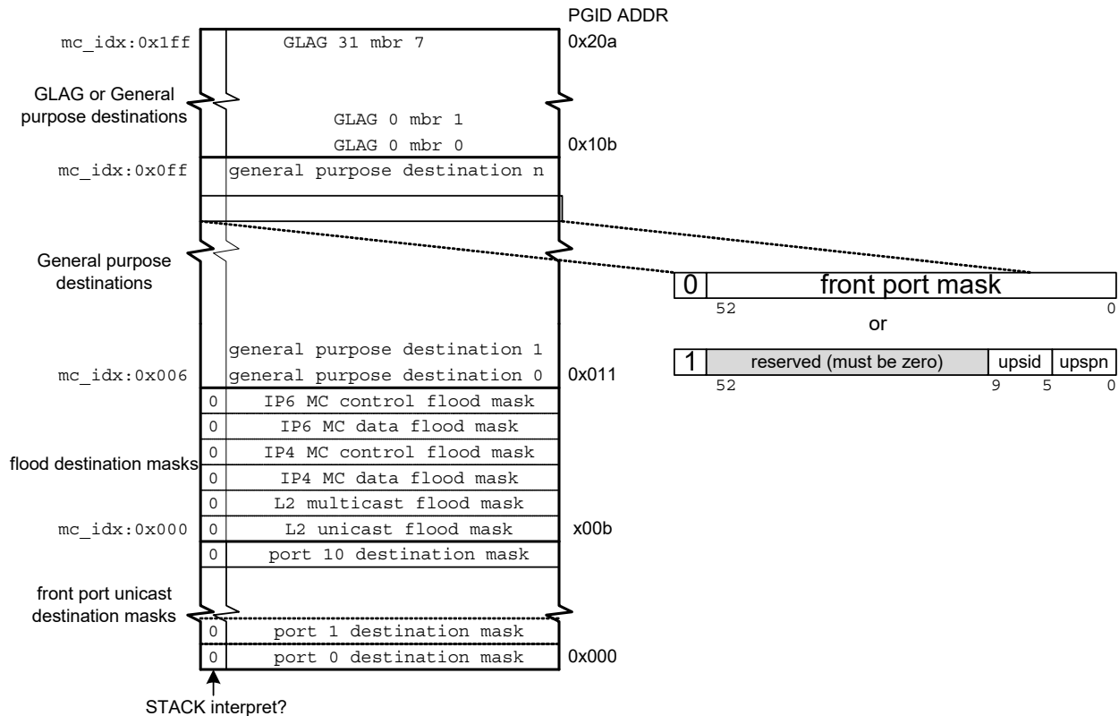
Figure 40 • PGID Layout
