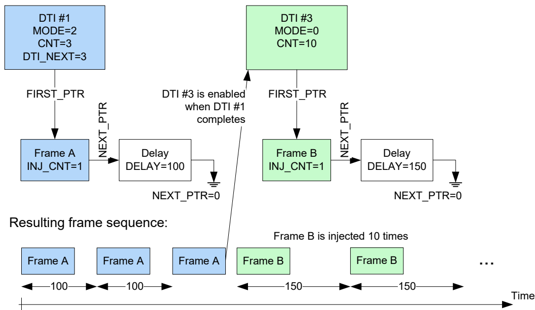
Figure 75 • DTI Concatenation
