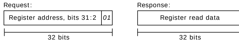
Figure 90 • WRITE Command
