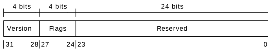
Figure 92 • VRAP Header Format
