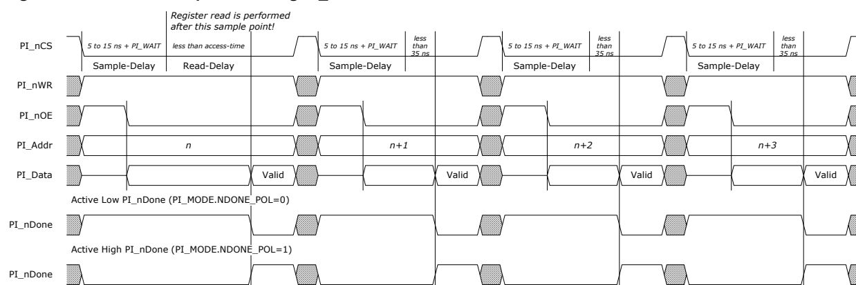
Figure 57 • PI Read Sequence Using PI_nDone
