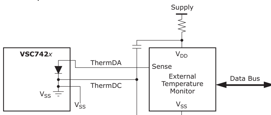
Figure 127 • External Temperature Monitor Connection
