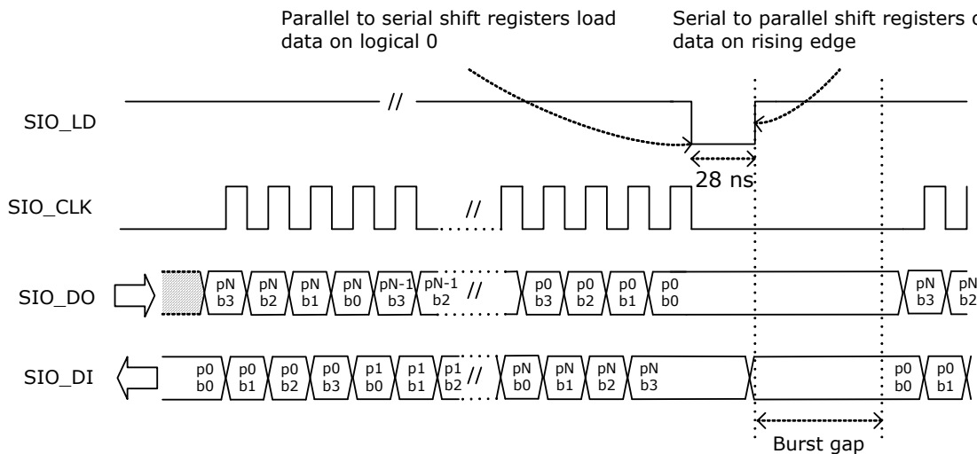
Figure 63 • SIO Timing
