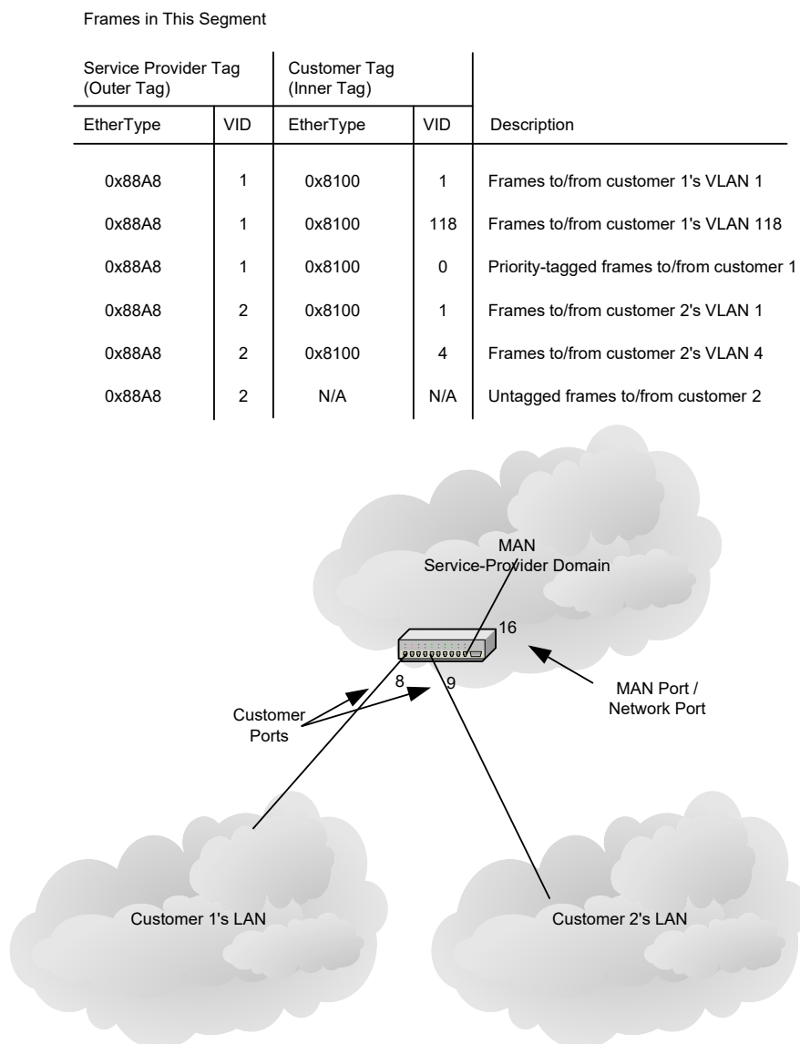
Figure 69 • MAN Access Switch Setup
