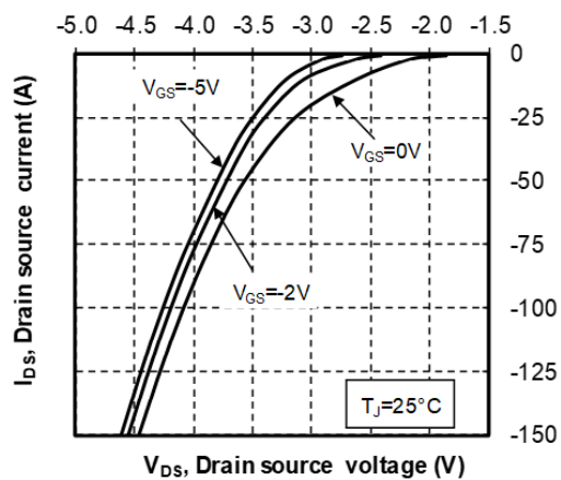
Figure 10 • Body Diode Characteristics, T_J = 25^\circ C
