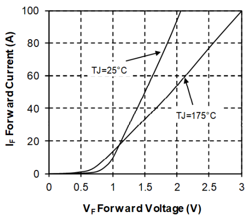
Figure 19 • Forward Characteristics
