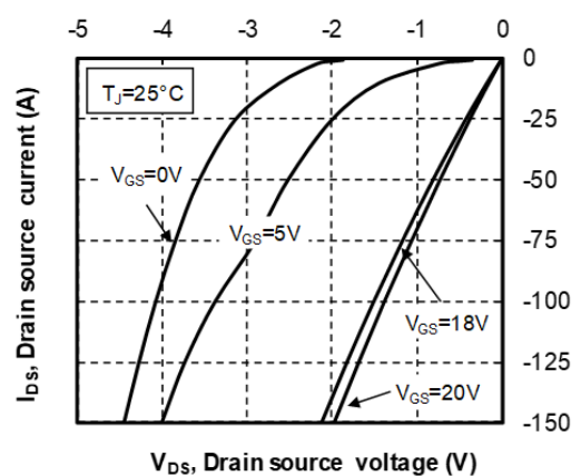
Figure 11 • 3 rd Quadrant Characteristics, T_J = 25^\circ C
