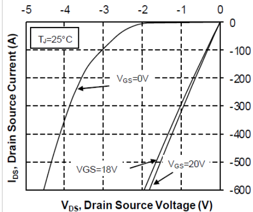
Figure 13 • 3 rd Quadrant Characteristics, T_J = 25^\circ C
