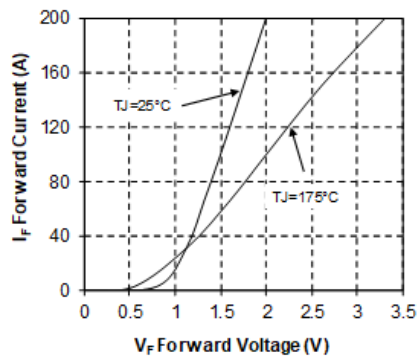
Figure 2 • Forward Characteristics
