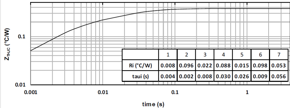
Figure 3 • Maximum Thermal Impedance
