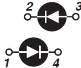
Figure 2 • Anti-parallel MSC2X50SDA170J
