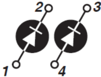
Figure 1 • Parallel MSC2X31SDA070J
