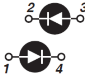
Figure 2 • Anti-parallel MSC2X100SDA070J
