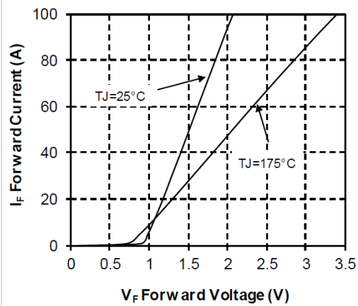
Figure 18 • Forward Characteristics
