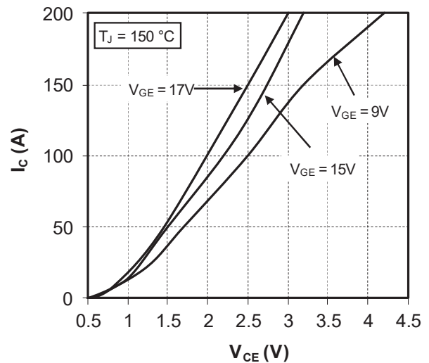
Figure 1-13. Output Characteristics, T_J = 150^{\circ}\text{C}
