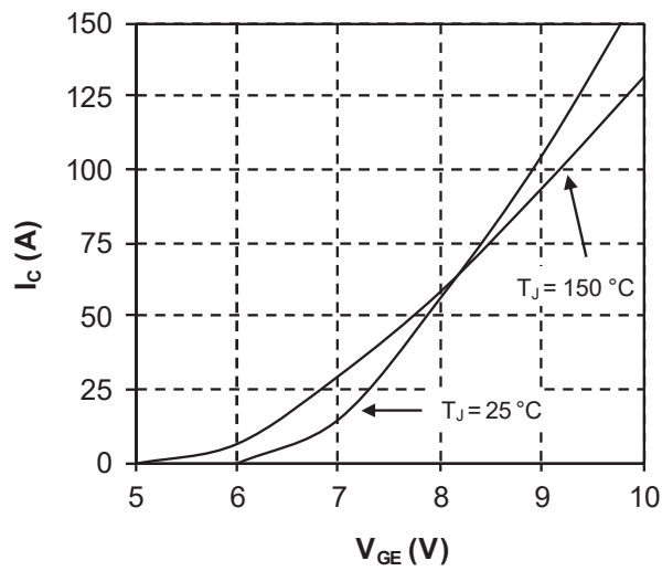
Figure 1-4. Transfer Characteristics
