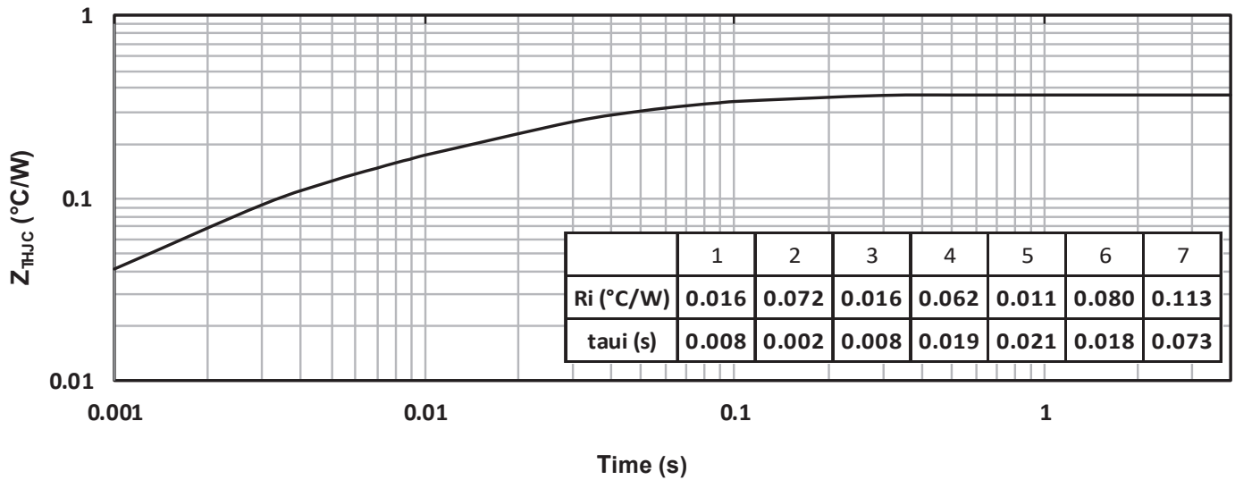
Figure 1-11. Maximum Thermal Impedance
