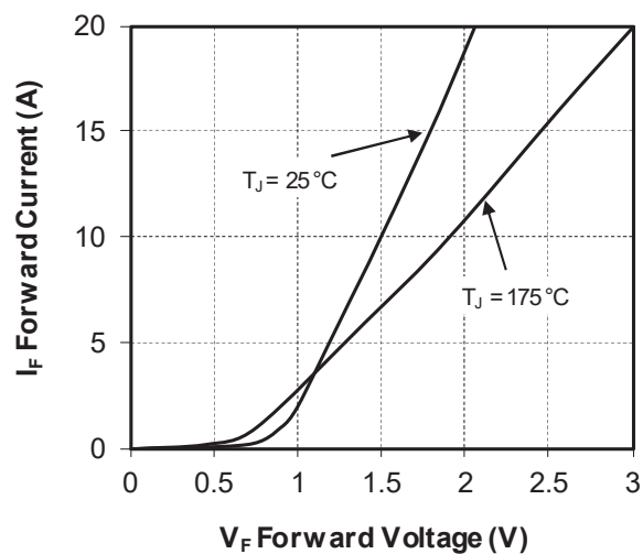
Figure 1-21. Forward Characteristics
