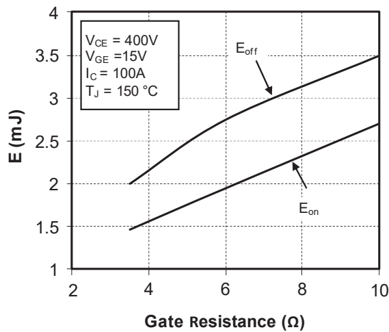
Figure 1-16. Switching Energy Losses vs. Gate Resistance
