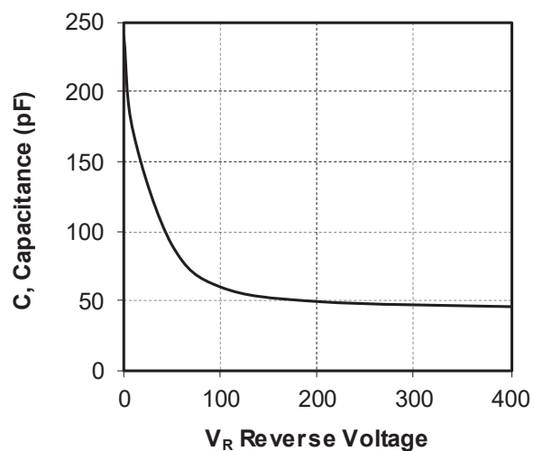
Figure 1-22. Capacitance vs. Reverse Voltage
