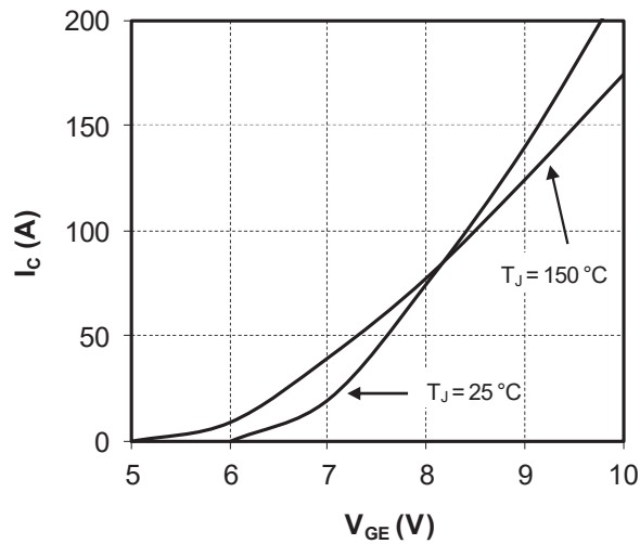
Figure 1-14. Transfer Characteristics
