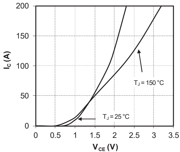
Figure 1-12. Output Characteristics, V_{GE} = 15\text{V}
