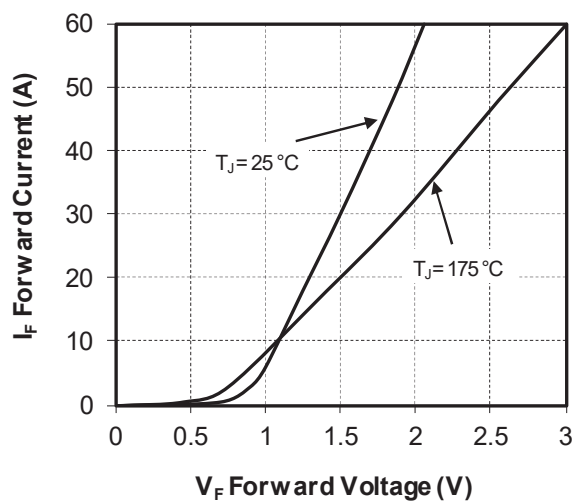
Figure 1-9. Forward Characteristics
