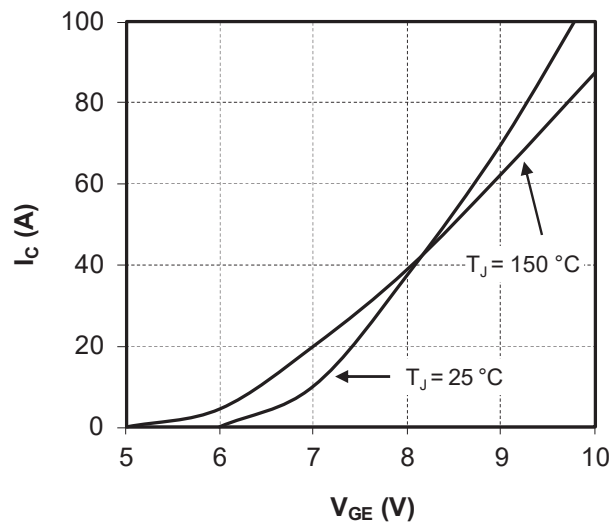
Figure 1-4. Transfer Characteristics
