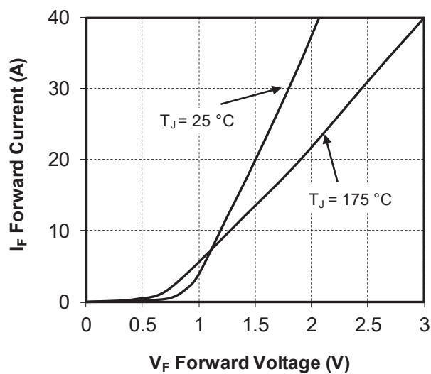
Figure 1-9. Forward Characteristics
