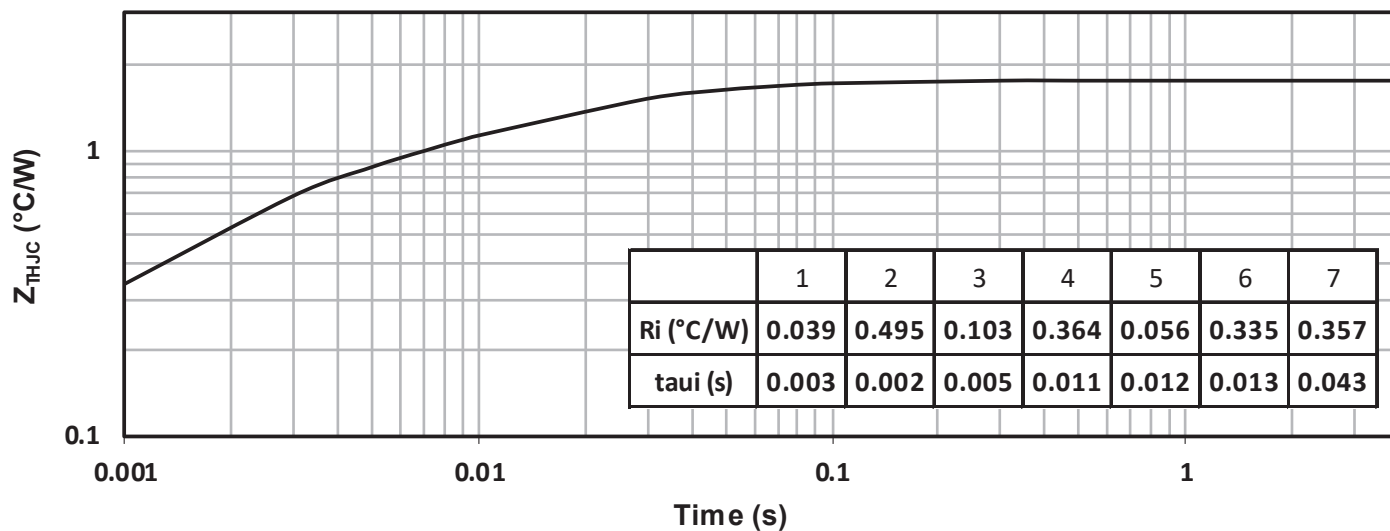
Figure 1-18. Maximum Thermal Impedance
