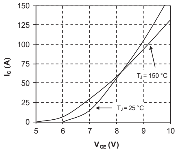
Figure 1-14. Transfer Characteristics
