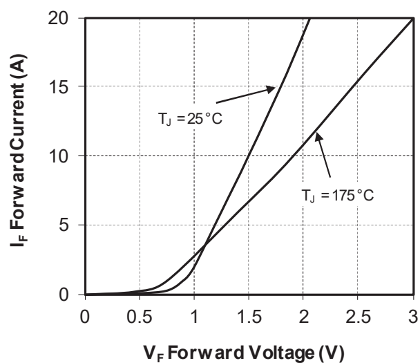
Figure 1-24. Forward Characteristics
