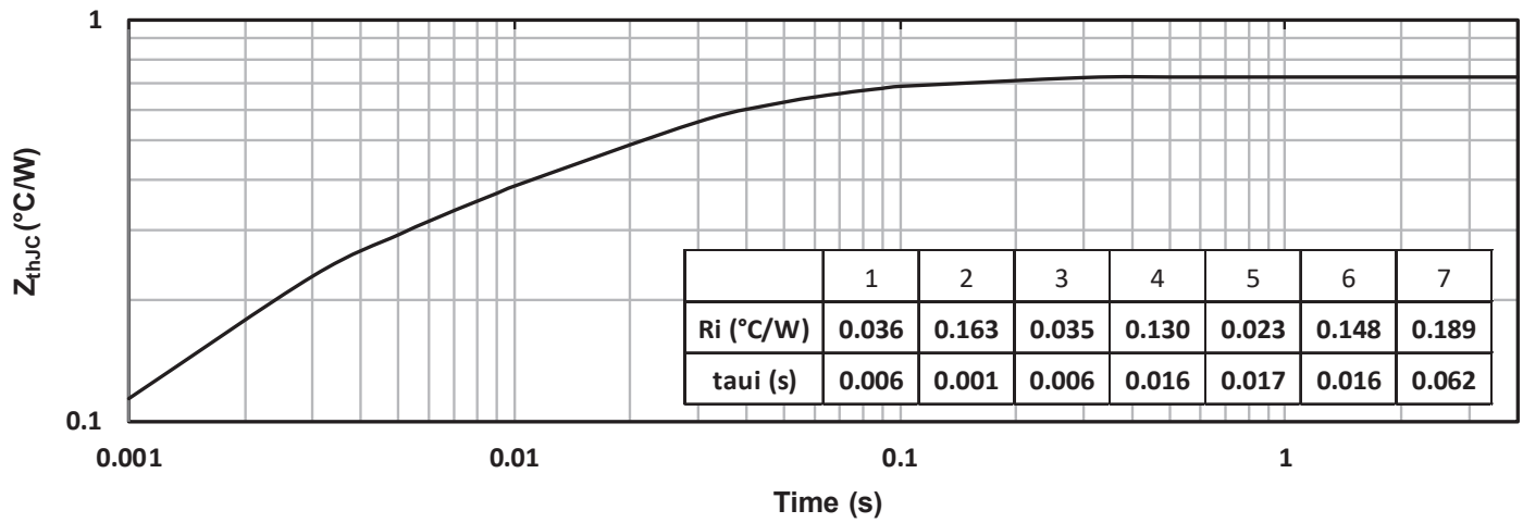
Figure 1-1. Maximum Thermal Impedance
