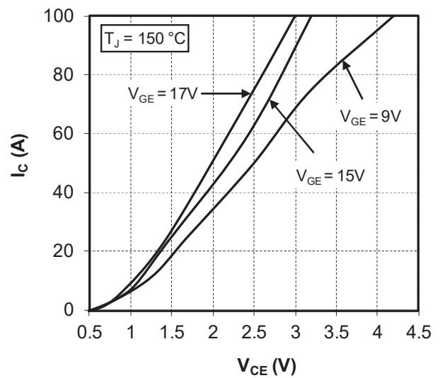
Figure 1-3. Output Characteristics, T_J = 150\text{ }^{\circ}\text{C}
