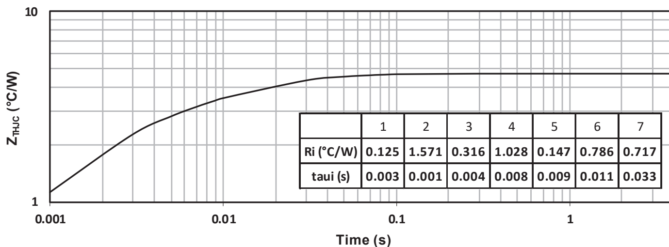
Figure 1-23. Maximum Thermal Impedance
