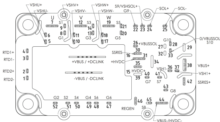
Figure 2. Pinout Location
