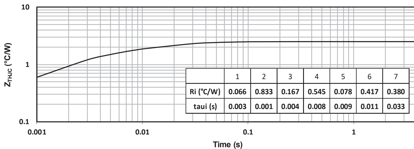
Figure 1-8. Maximum Thermal Impedance
