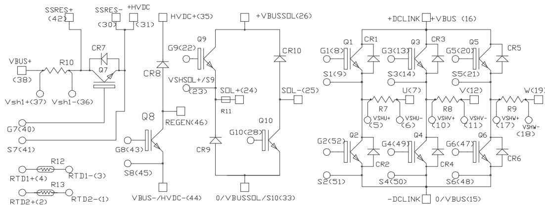
Figure 2. Pinout Location
