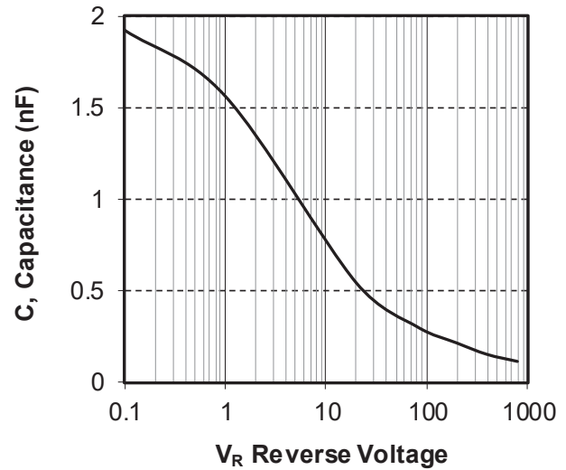
Figure 1-10. Capacitance vs. Reverse Voltage
